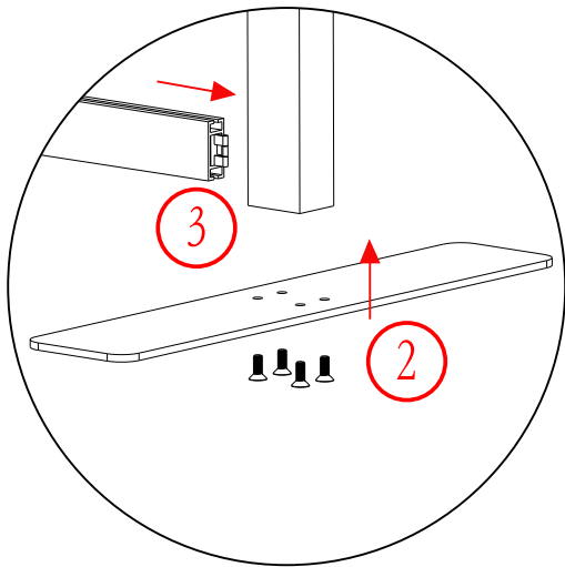
Base and Horizontal Pole Set-up
