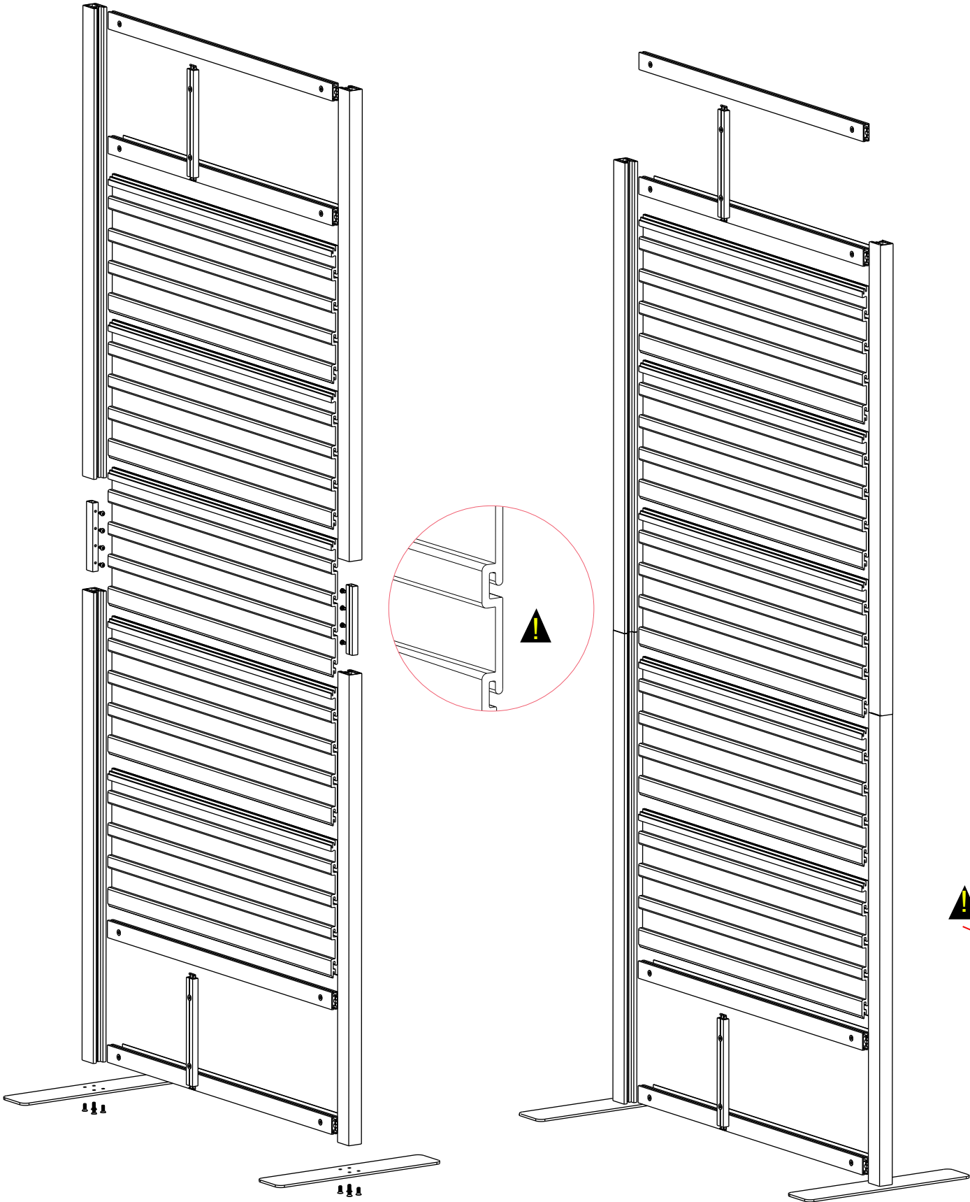
Slide Slatwall Panels into the frame
